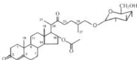
SN-3 (C 35 H 54 O 10 )
