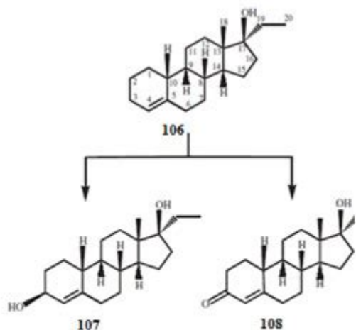
Fig. 21: Biotransformations of Ethylestrenol (106) by Rhizopus stolonifer .
